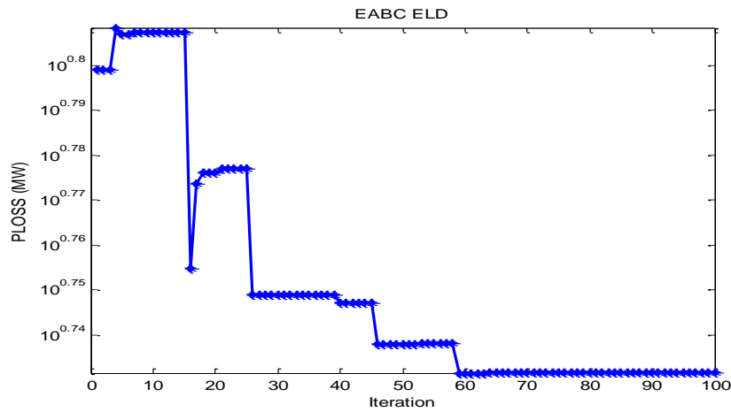
Figure6. the curve of system loss based on the number of repetition
