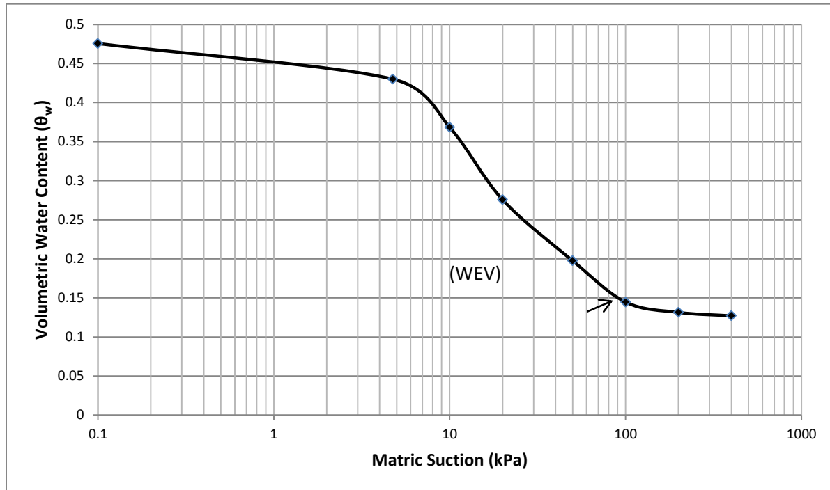
Figure.12 Wetting water retention characteristic curve
