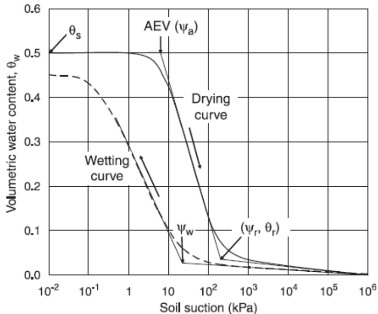
Figure1. Idealized Water Retention Characteristic Curve
