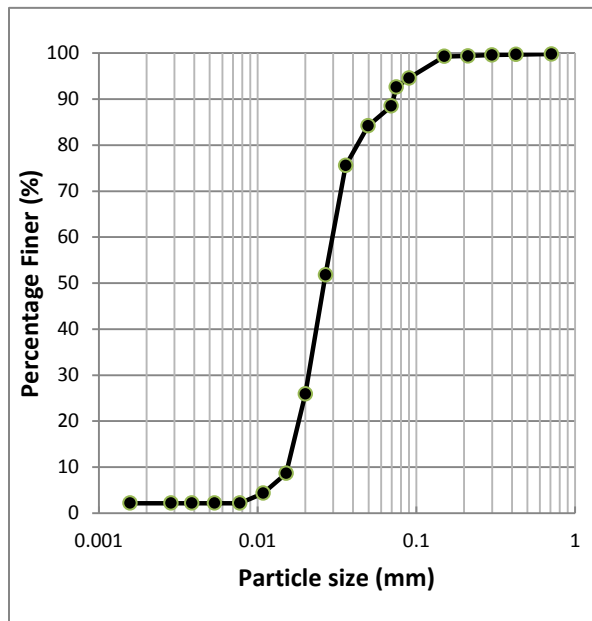
Figure 3. Grain size distribution curves of representative pond ash sample
