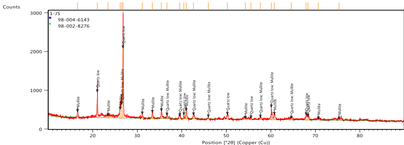
Figure 5(c). X-ray diffraction (XRD) of finer ash material (RP-O)
