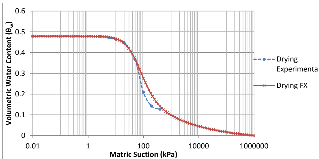
Figure.9 Measured and Predicted Drying WRCC using FX Model
