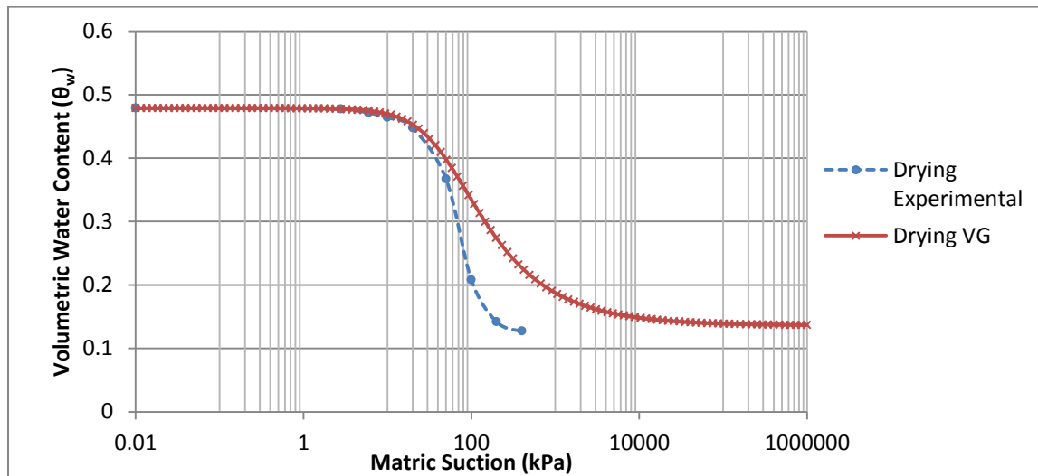
Figure.10 Measured and Predicted Drying WRCC using VG Model
