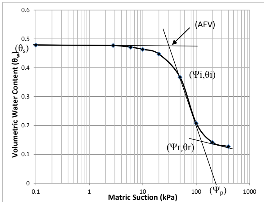
Figure.8 Drying water retention characteristic curve
