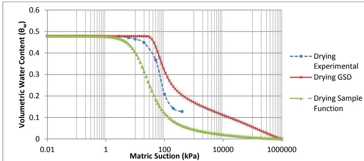
Figure.11 Measured and Predicted Drying WRCC using Estimation Method
