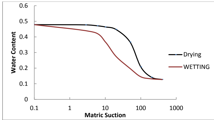
Figure.14 Hysteresis of WRCC of pond ash
