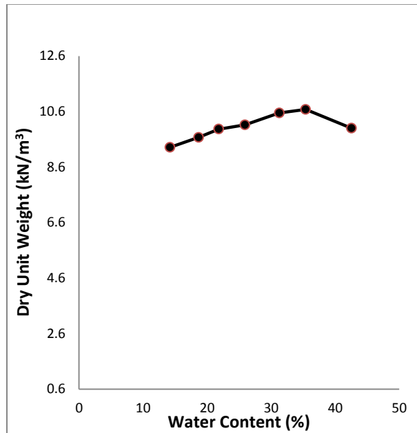
Figure 4. Compaction curve of Ropar Pond ash
