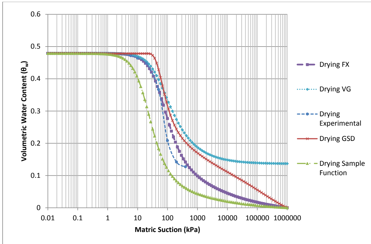
Figure.13 Measured and Predicted Drying WRCC using different methods
